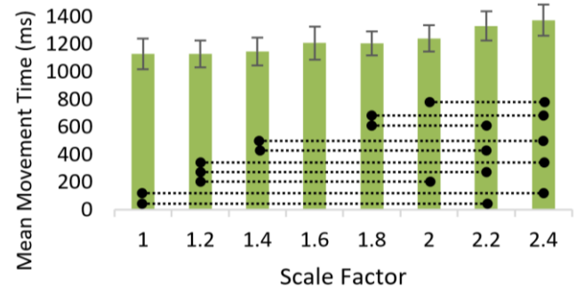
Figure 7: Mean MT for each SF. Error bars show 95% CI.
