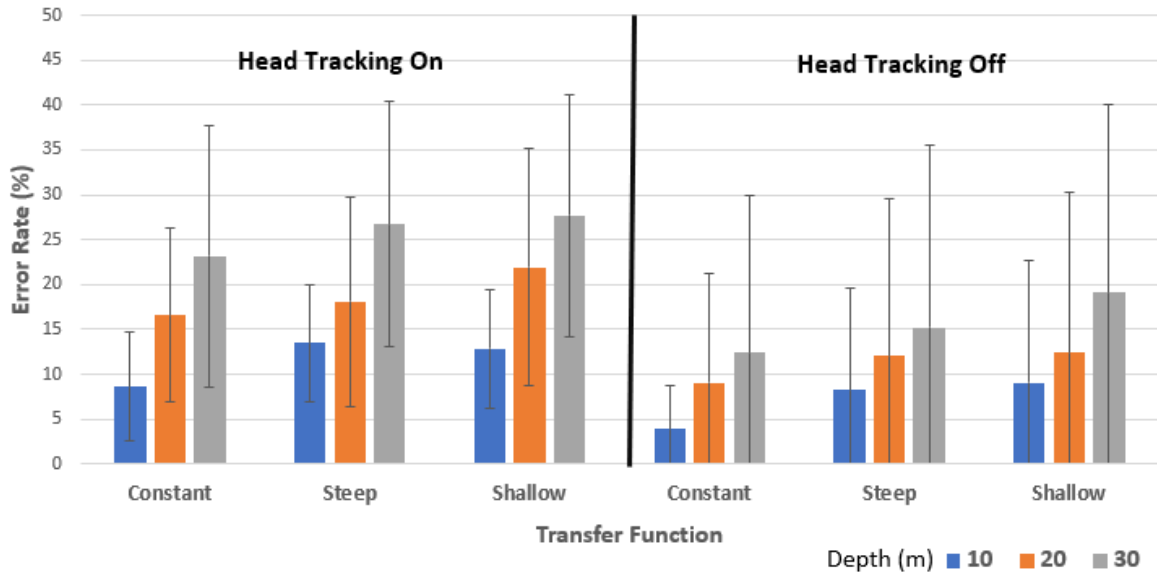
Figure 14: Error Rate on Depth. Error bars show \pm 1 SD.
