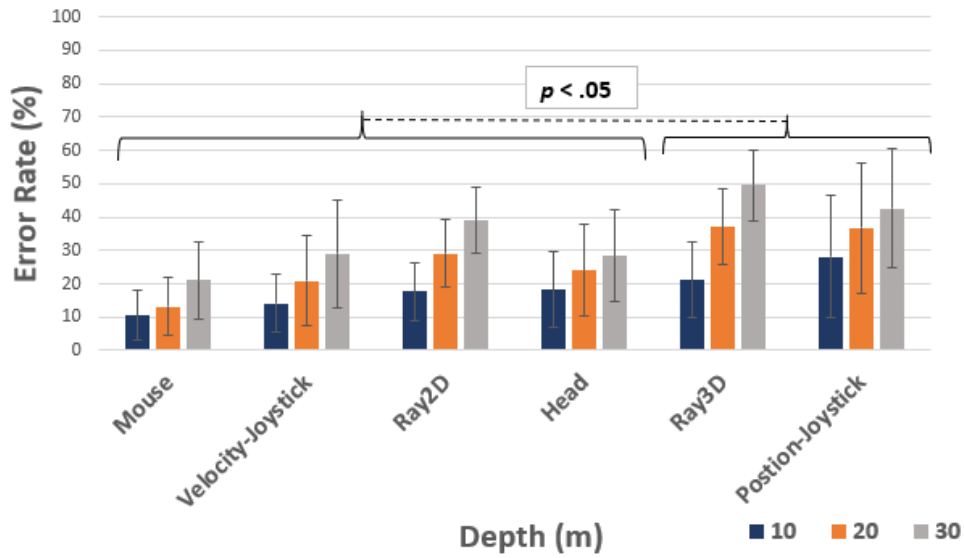
Figure 9: Error rate by controller and depth. Error bars show \pm 1 SD.
