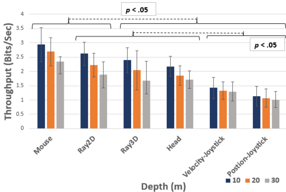
Figure 7: Throughput by Depth. Error bars show \pm 1 SD . Statistical groups (i.e., controllers that are not significantly different) are indicated with curly braces, with dashed lines showing significant differences to other groups via the Scheffe test.
