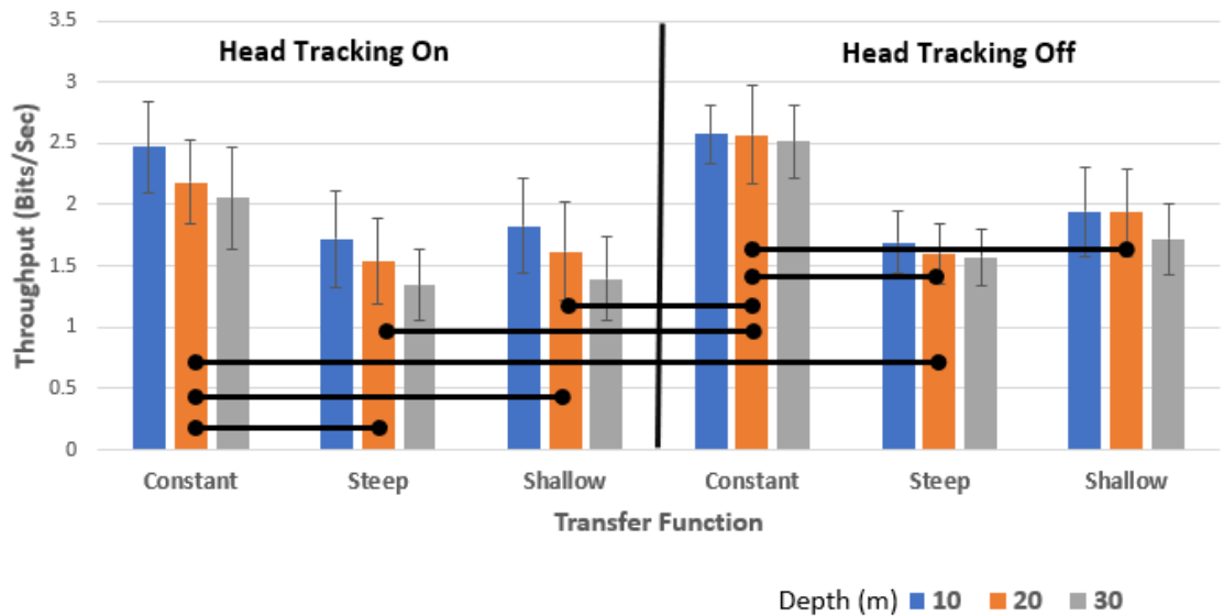
Figure 12: Throughput on Depth. Error bars show \pm 1 SD.
