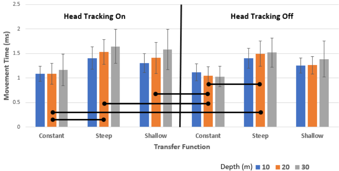
Figure 13: Movement Time on Depth. Error bars show \pm 1 SD. Note: bars show significant pairwise differences between transfer functions, but not depths.
