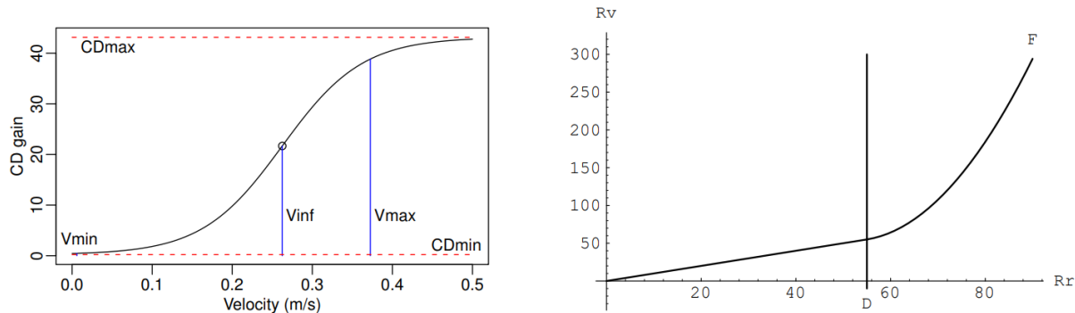
Figure 2: Curves showing two different acceleration functions. Left: Nancel 2015 [27], Right: Poupyrev 1996 [32].
