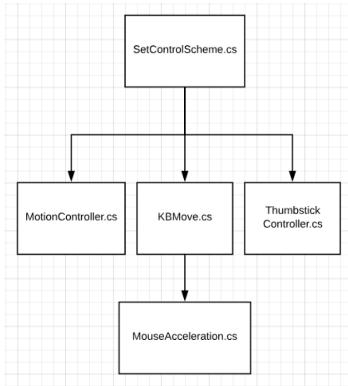
UML diagram for cursor movement via input devices
