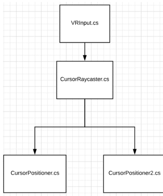
UML diagram for cursor positioning and rendering classes
