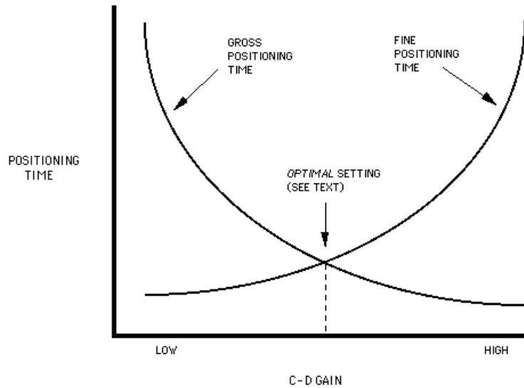
Figure 1: The relationship between CD gain and selection time. Fine positioning becomes more difficult with high gain (due to overshooting targets) while coarse positioning takes longer with low gain due to excessive clutching. Figure reproduced from Jenkens and Connor [17]
