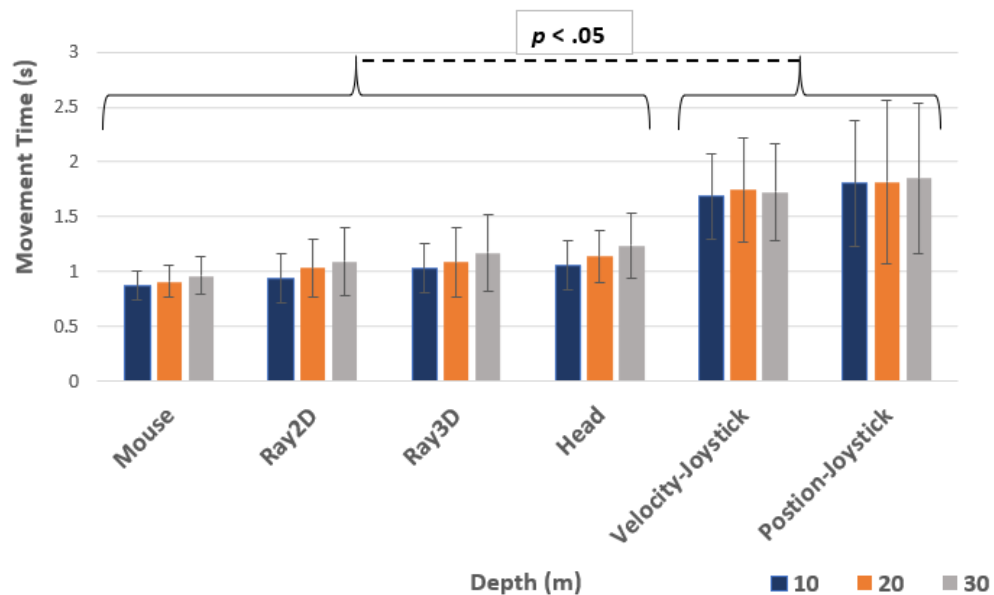
Figure 8: Movement time by controller and depth. Error bars show \pm 1 SD.
