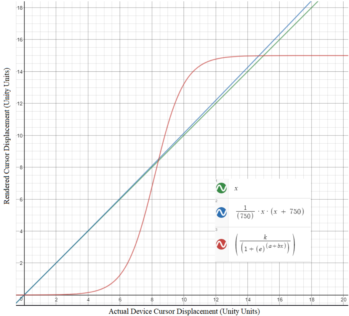
Figure 11: Graph of both Transfer acceleration functions used along with constant acceleration as a baseline (Green: Constant, Blue: Shallow, Red: Steep).
